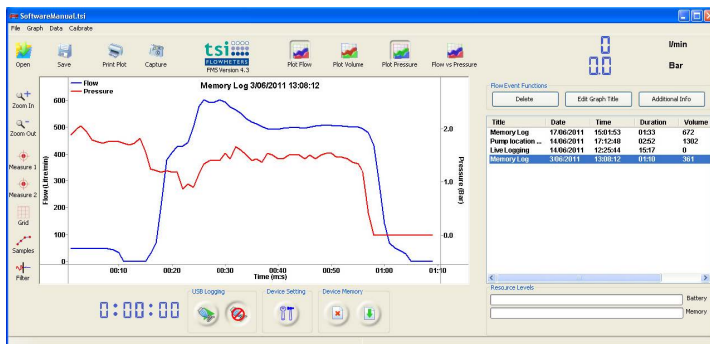
FMS Software
